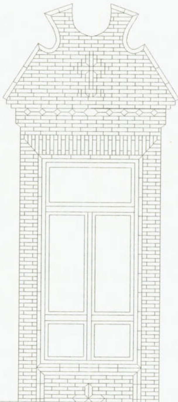
دetailed drawing of a brick window (دetailed drawing of a brick window)
